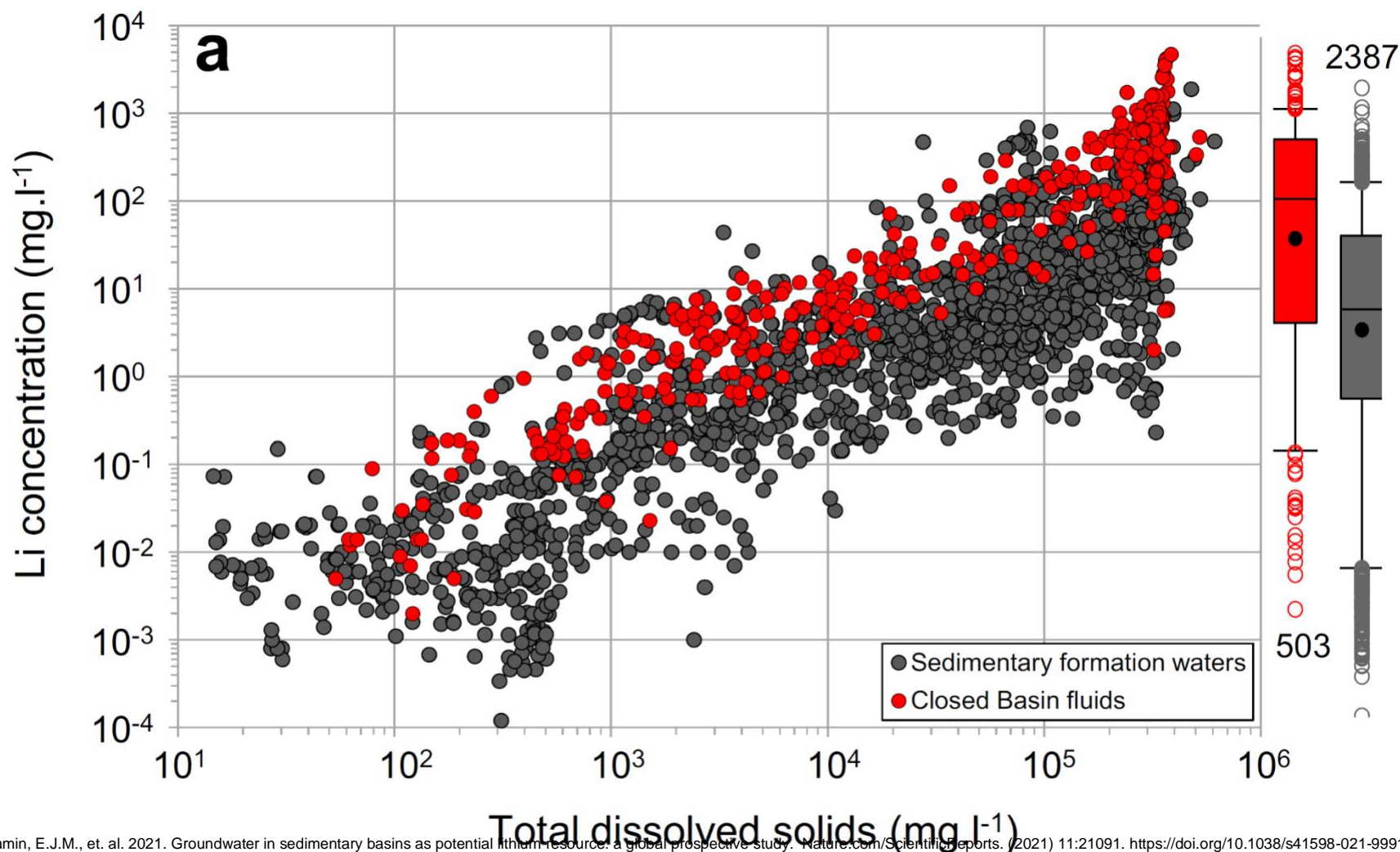
Figure 2 – Lithium concentration in formation waters from sedimentary basins and closed basin brines worldwide; lithium concentration vs. total dissolved solids
